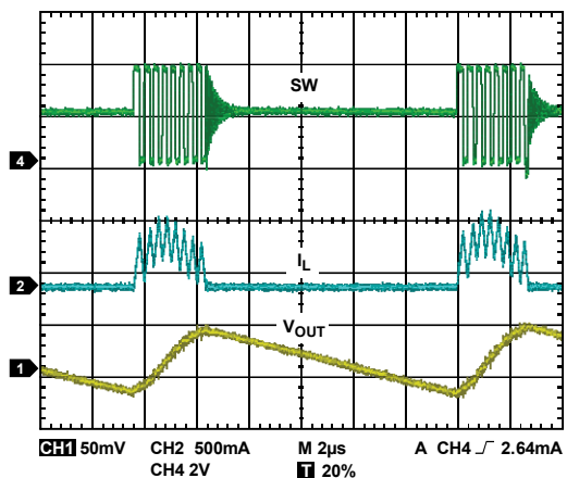
Figure 27. Typical Power Save Mode Waveform, 50 mA
