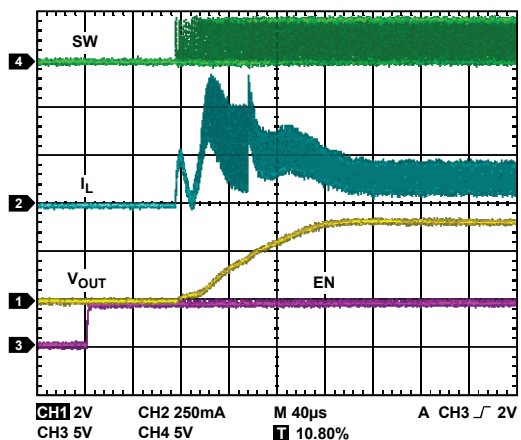
Figure 26. Start-Up, V_{OUT} = 3.3\text{ V} , 150 mA
